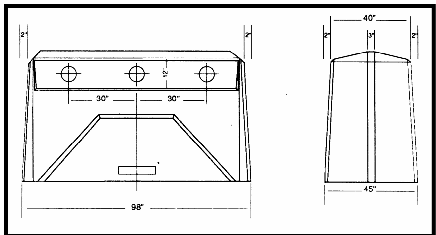
Outside dimensions of eco•tainer Tri-Cart
